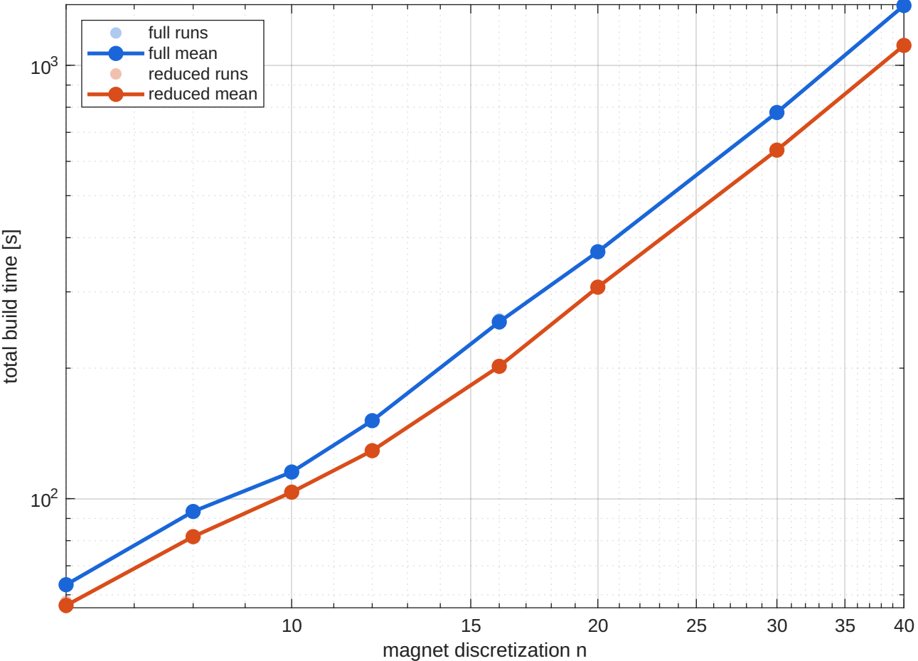
Build time vs n (log-log)
